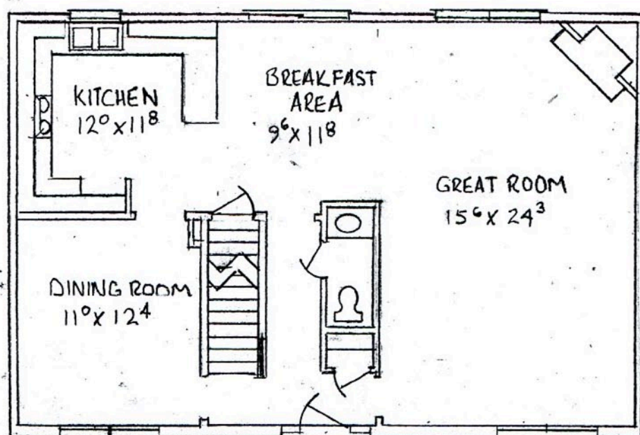
1st Floor - 969 sq ft
